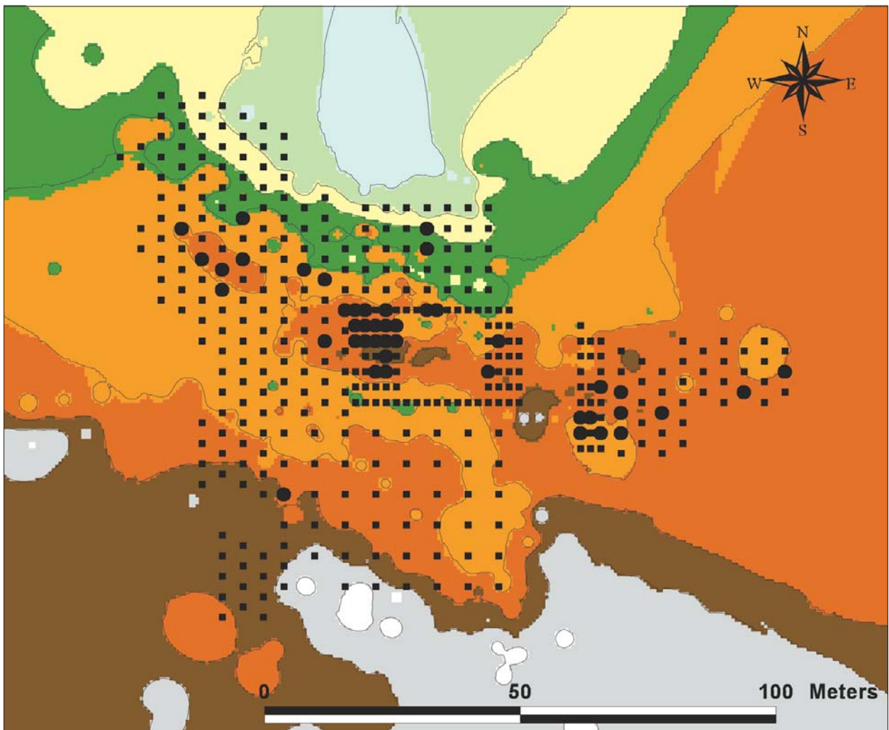
Fig. 8. Digital elevation model of Research area 1: Filled circles are positive test-pits, filled squares negative test-pits. Elevation ranges from green and blue (lowest) to grey and black (highest). The dwelling depression and the activity areas are situated midway between the highest and the lowest point.
